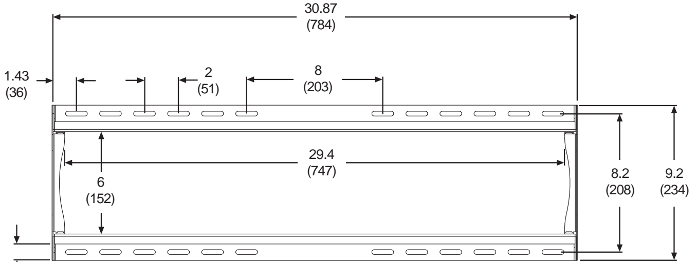
WALL PLATE DETAIL
