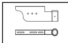
Side Mount Bracket Part #2349
