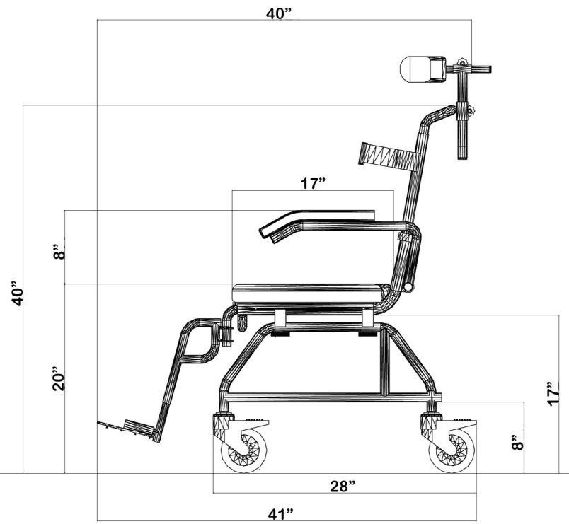
SB3 showerbuddy dimensions drawn 27/02/2008
