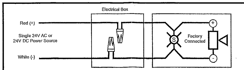
Figure 2. Connecting the Horn and Strobe
