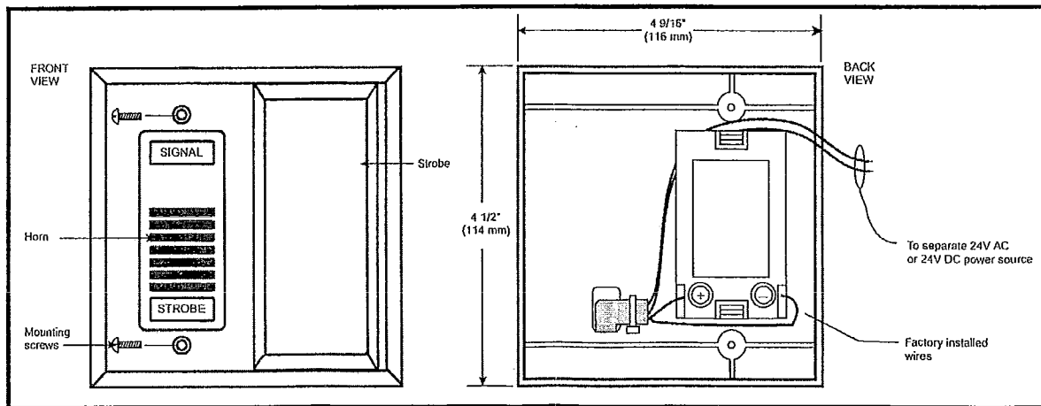
Figure 1. Details of Horn/Strobe
