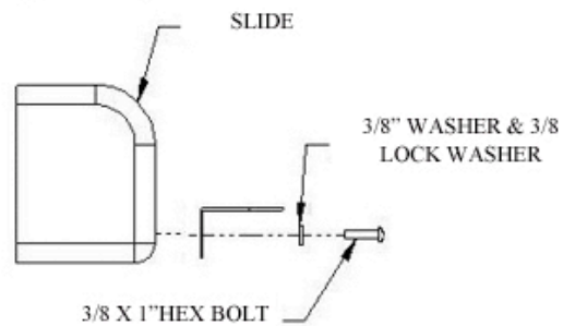
VIEW D
