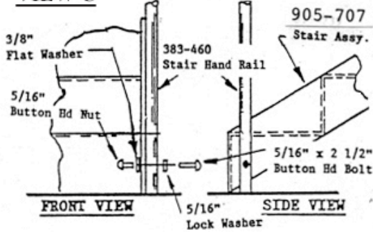
VIEW C
