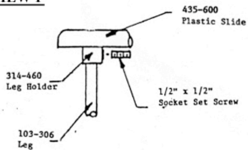
VIEW F
