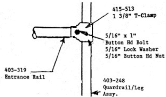
VIEW B
