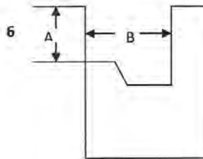
Rollout Gutter
