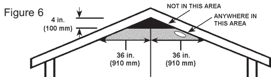
Figure 6: RECOMMENDED SMOKE ALARM LOCATION IN ROOMS WITH SLOPED, GABLED, OR PEAKED CEILINGS.
