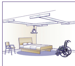
94003: An x-y system without posts and with 4 wall brackets
