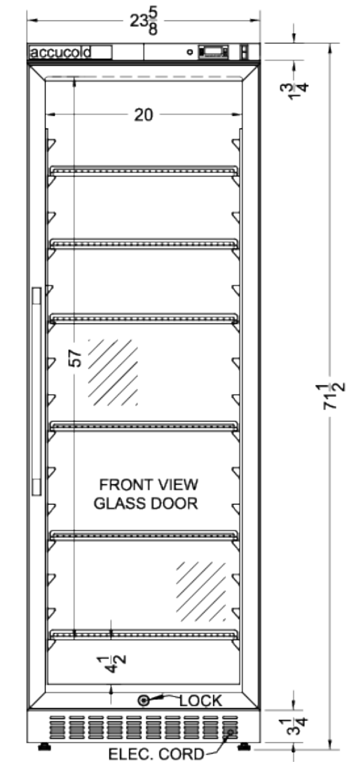
Puretherm Warming Cabinet
